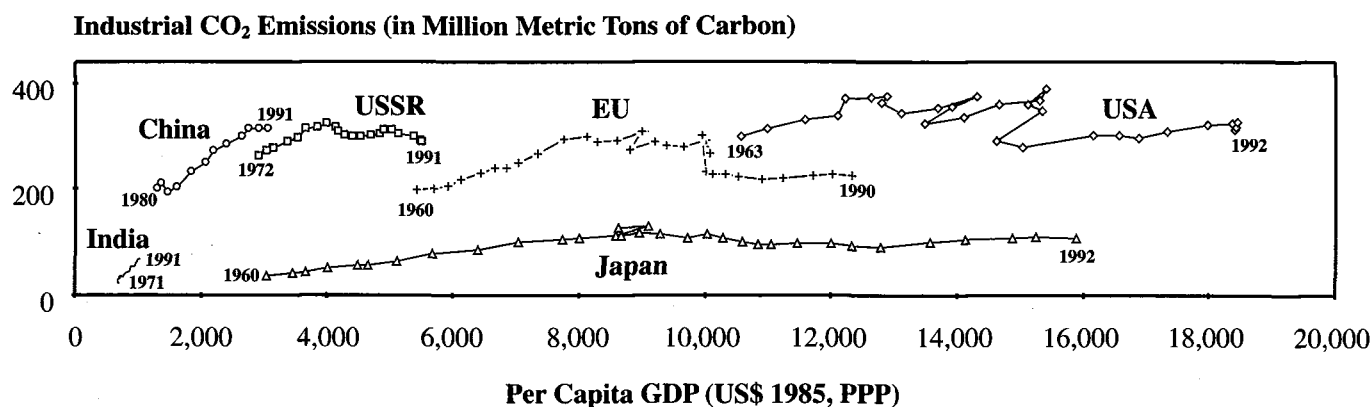
Figure 10: Fossil fuel CO 2 development path for the industrial sectors of the United States, the 15 nations that now comprise the European Union (less the former East Germany), Japan, China, India, and the former Soviet Union. The industrial sector is as defined by OECD, plus CO 2 associated with refineries and the fraction of electricity that is used by industry. The CO 2 values are from OECD (1994), and the ppp values are from Sommers and Heston (1991, 1994); see Chapter 20 for complete citations.
