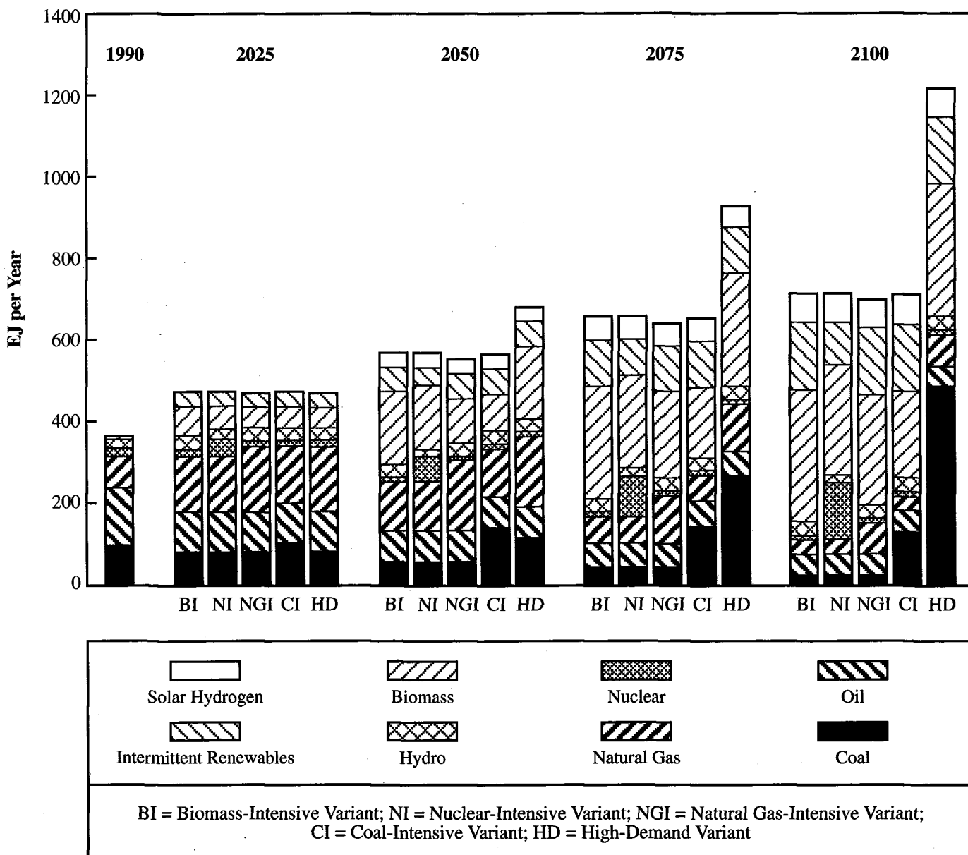
Figure 19-8: Global primary energy use for alternative LESS constructions.
