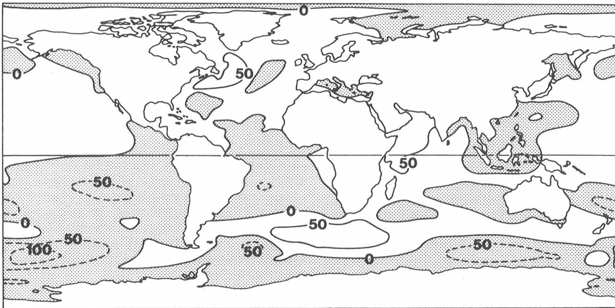
Figure 8-4: Global variations of sea-surface topography (in mm) due to dynamic effects relative to the global mean sea level, as obtained from a transient experiment of increasing carbon dioxide concentrations using a coupled ocean-atmosphere GCM. The results are for years 66–75 of the model run (but cannot be ascribed to a future calendar date). The stippled areas on the map show sea-level rises that are less than the global average (after Gregory, 1993).
