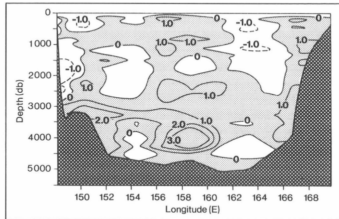
Figure 8-3: The difference of the potential temperature between 1967 and 1990 across 43°S between Australia and New Zealand. The unit of the difference has been normalized by the root-mean-square variability (after Bindoff and Church, 1992).
