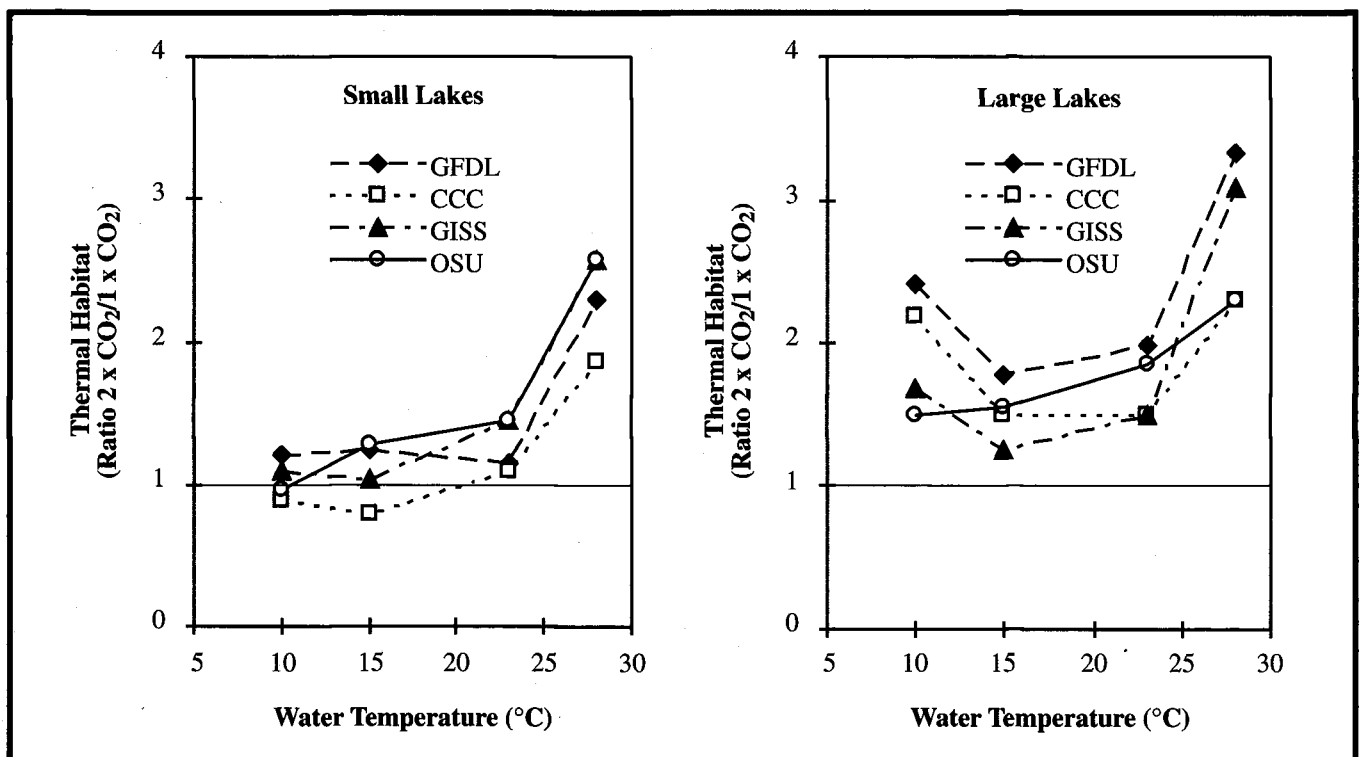
Figure 10-9: Simulated changes in thermal habitat in small (Crystal and Sparkling) and large (Michigan, Mendota, and Trout) stratified temperate lakes for cold- (10 and 15°C), cool- (23°C), and warm-water (28°C) fish under a 2 x CO 2 climate with four GCMs (GFDL, CCC, GISS, and OSU), as modified from Magnuson and DeStasio (1996).
